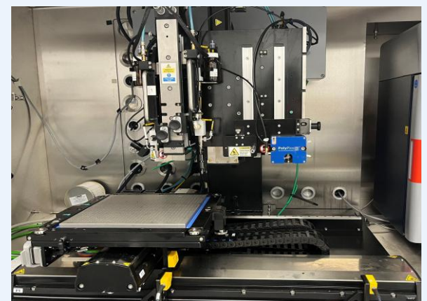
Pilot Line Integrated PolyPico Unit
