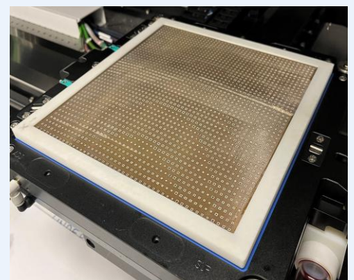
Large area Printing of Antenna Array
